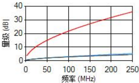
插入损耗
