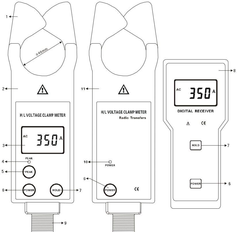
ETCR9000
