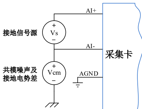
图 4-5-5 接地信号源的差分 (DIFF) 连接
