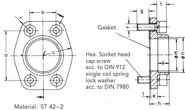
Material: ST 42-2
