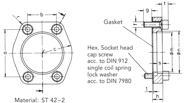
Material: ST 42-2
