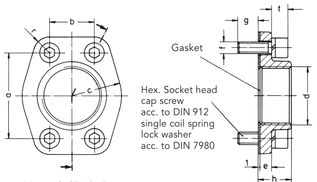
Material: ST 42-2
