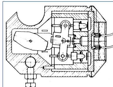
Section through type H4 switch mechanism
