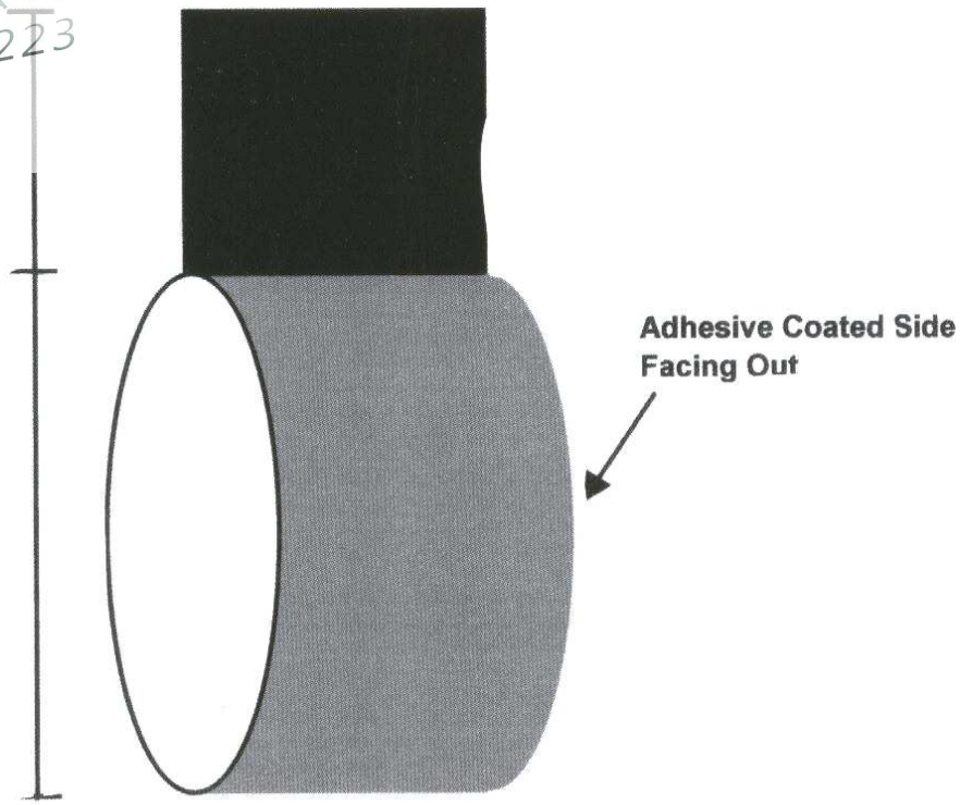
Figure1. Specimen loop - Test Method A.
