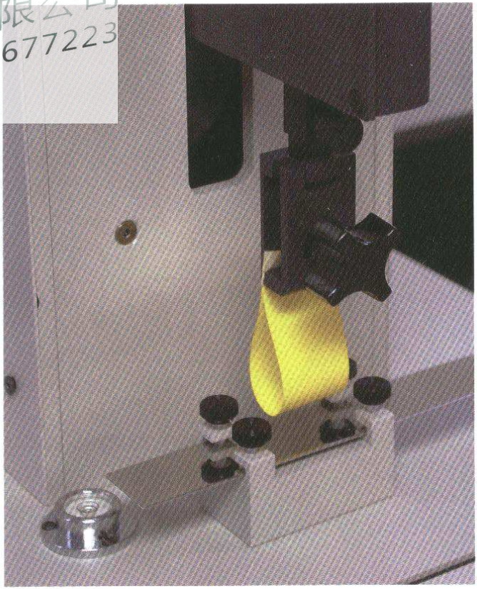
Figure 5. Loop fixture mounted in loop tack tester.
