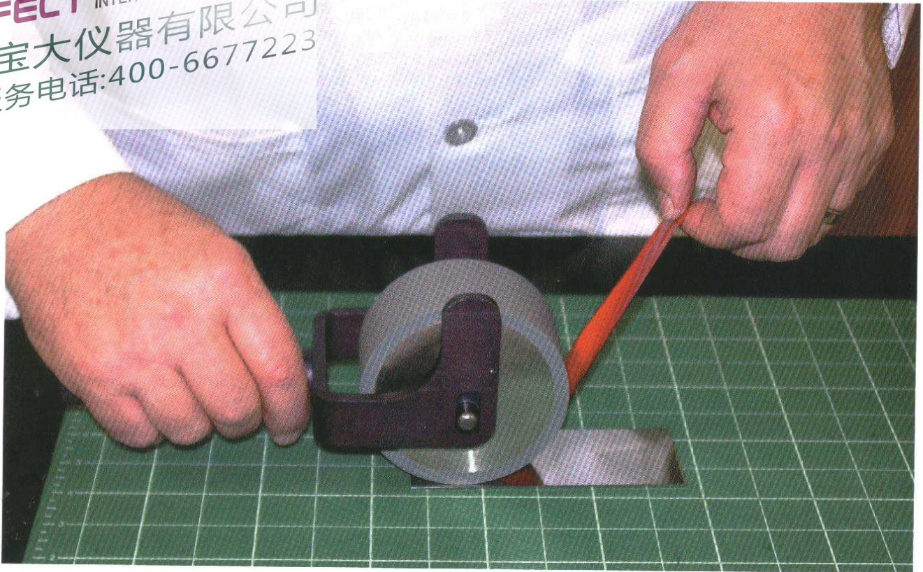
Figure 1. Hand operated roll down unit.
