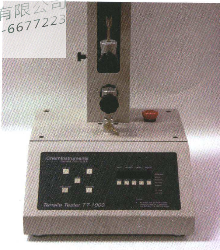
Figure 3. Tensile tester.
