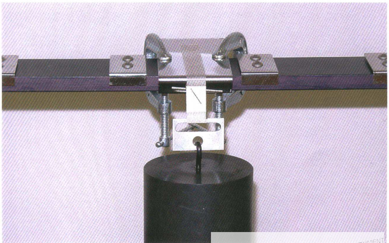
Figure 3. Shear adhesion sample in test stand (initial)
