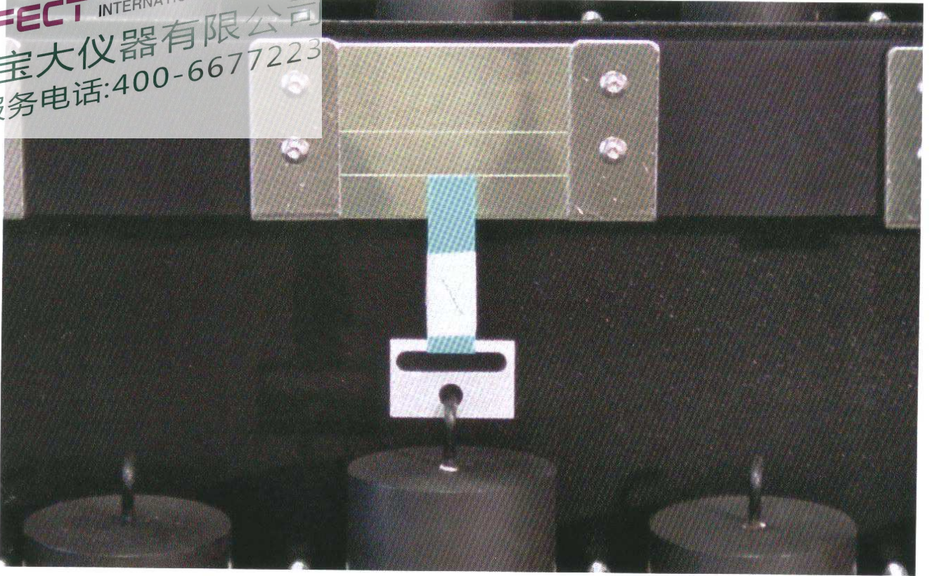
Figure 4. Shear adhesion sample in test stand (final).
