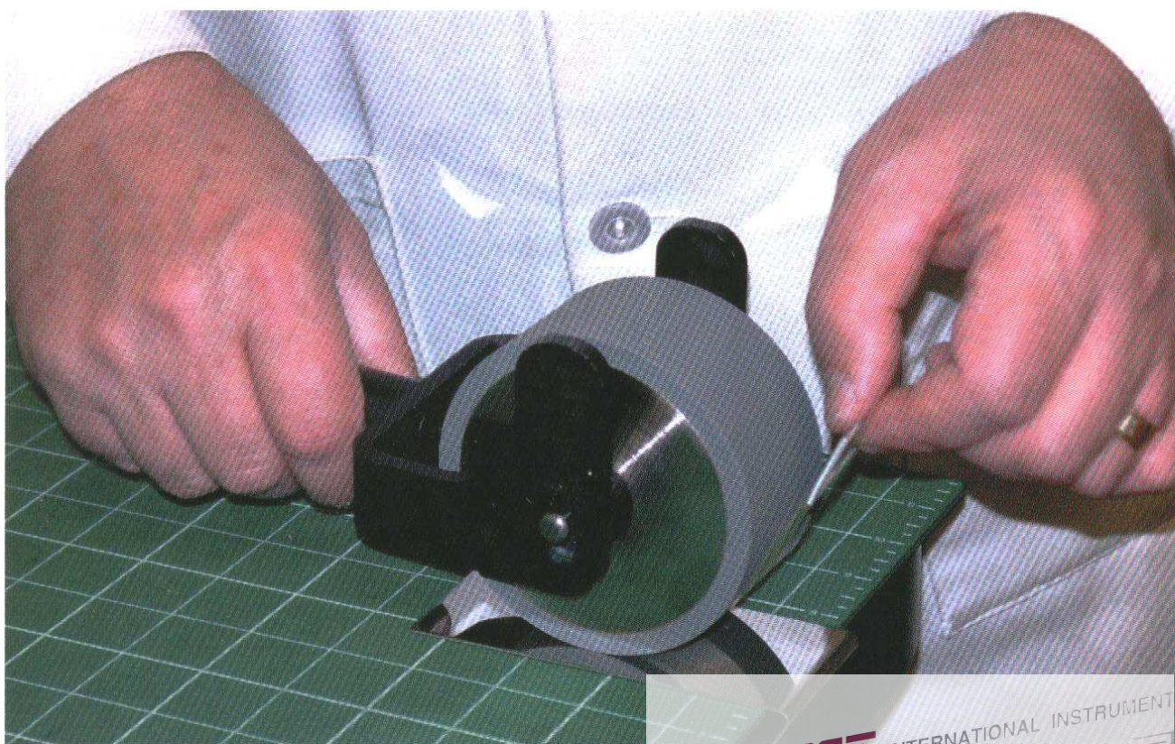
Figure 1. Controlled roll down shear adhesion sample preparation
