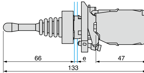
XD4-PA..4
