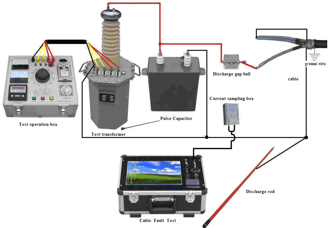
Red flash method current sampling physical wiring diagram
