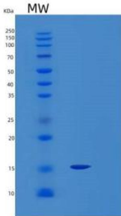
Figure . SDS-PAGE
