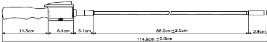
Video Borescope with Orange Rubber Cover
