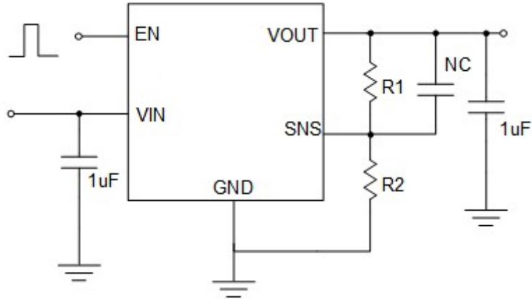
Figure 4: Adjustable output voltage LDO application circuit by JC2306N-08S5
