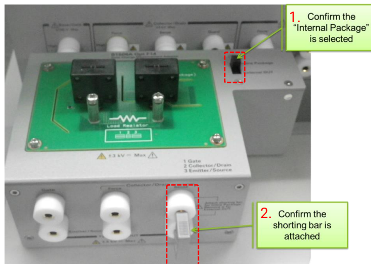
Figure 5-41 TO-device fixture calibration for Qg measurement.
