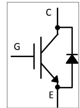
FGA180N33ATD IGBT
