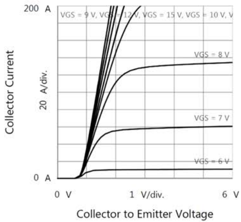
Output Characteristics
