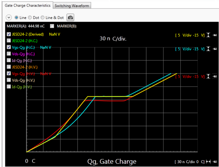
Figure 5-24 A Qg measurement example of a Vgs from -15 V to +15 V.
