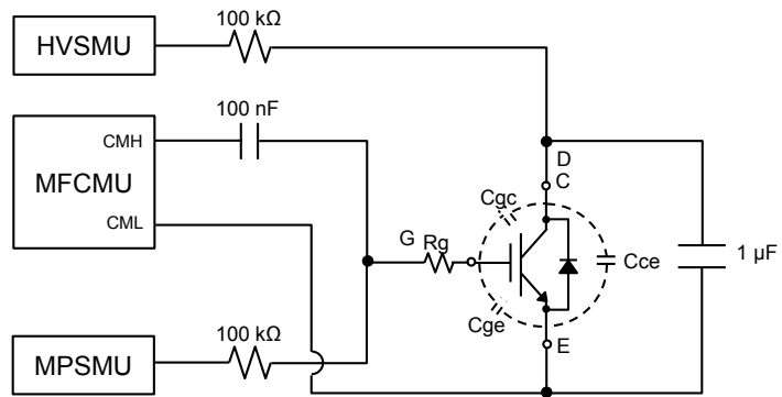
R g Measurement circuit for IGBT with collector biased condition
