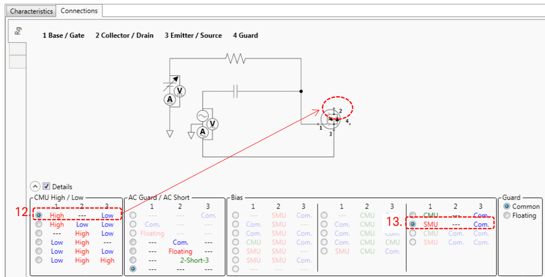
Figure 4-32 Making the collector/drain terminal open for Rg measurement.
