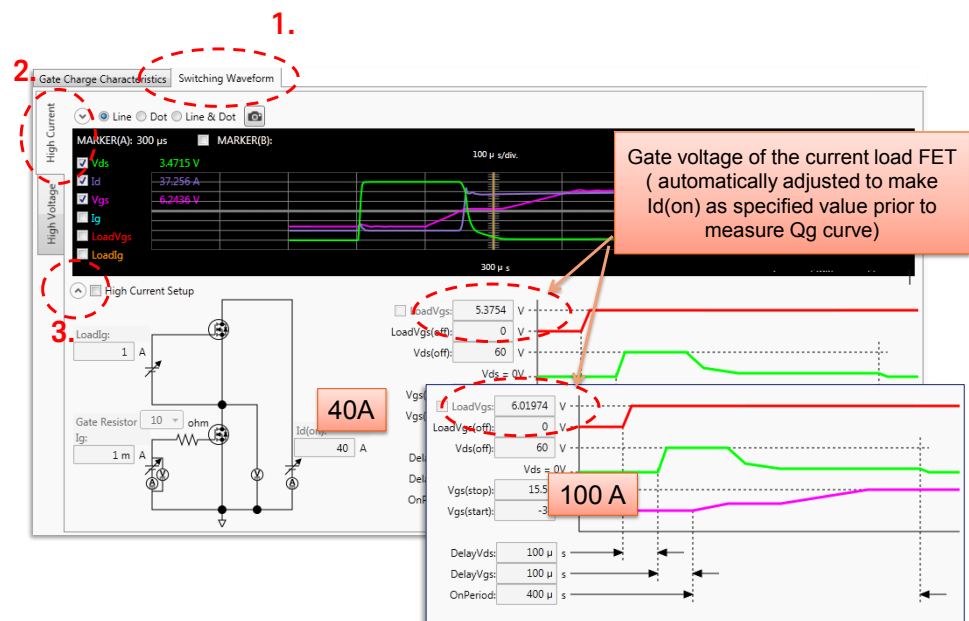
Figure 5-16 To monitor the setting of the current load FET.
