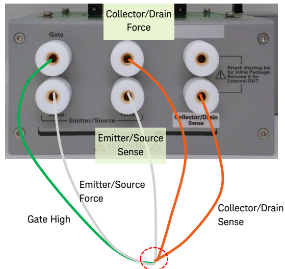
Figure 5-48 Module device's short calibration.
