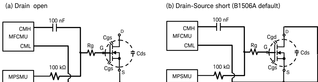
Figure 4-15 Rg measurement for power MOSFET
