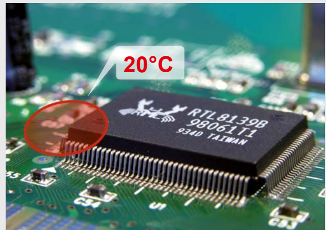
Spot size chosen too big which results in a measurement error
