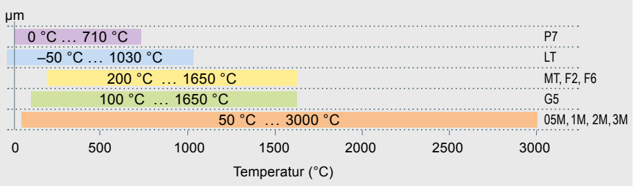
Display of temperature over wavelength for the devices of the high performance series
