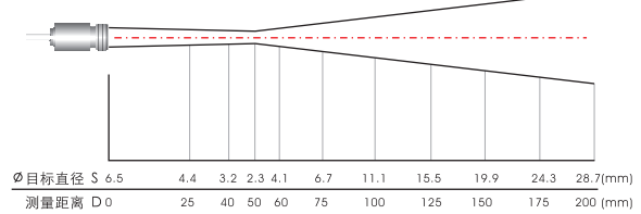
Optics CT LT CF, D:S=22:1 (远距离=6:1)
