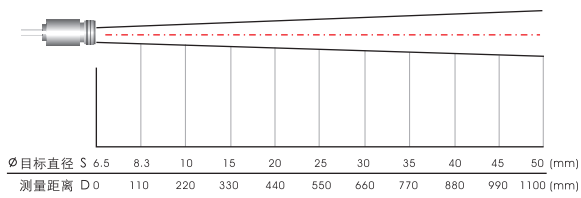
22:1探头
