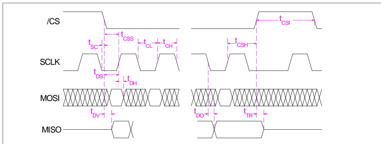
Fig. 5: Timing diagram
