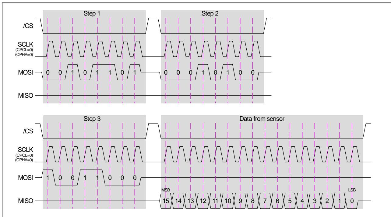
Fig. 5: SPI data transfer
