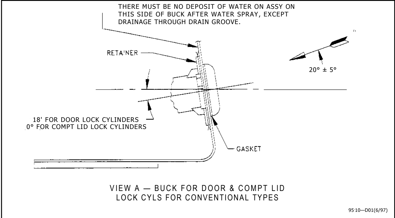
FIGURE 1D - BODY TEST POSITION FOR DOOR AND REAR COMPARTMENT LOCK CYLINDER
