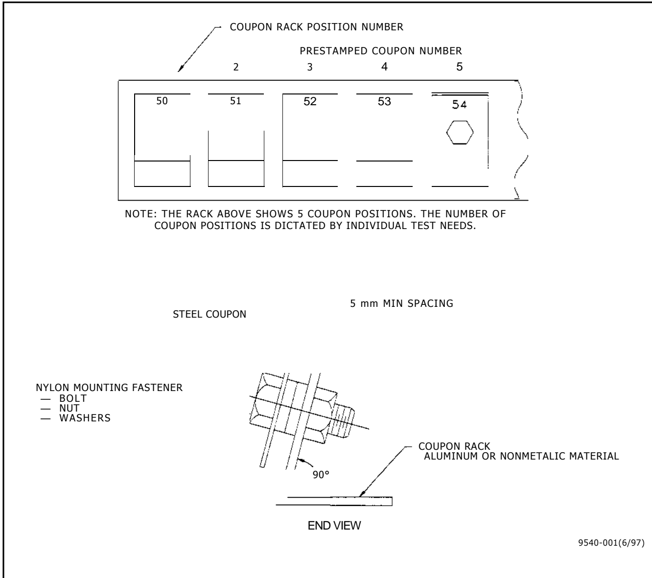
FIGURE 1 - COUPON RACK ASSEMBLY
