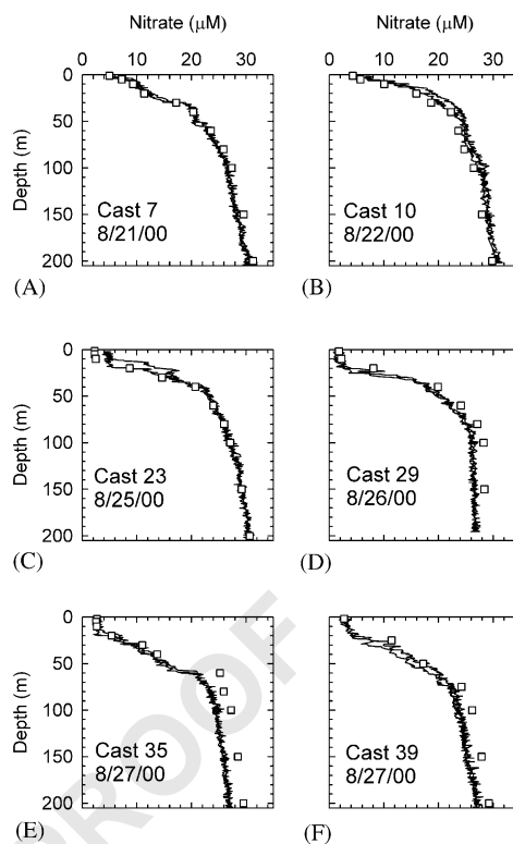
Fig. 5. Vertical nitrate concentration profiles calculated from a series of hydrocasts in Monterey Bay to 200 m depth. Up and down casts are shown. Nitrate concentration profiles determined with an Alpkem RFA autoanalyzer in water samples collected on the up cast are plotted as open squares.
