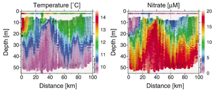
Fig. 7. (A) Temperature and (B) nitrate determined with ISUS and an FSI MicroCTD mounted on a SeaSciences Acrobat undulating vehicle. Nitrate and temperature data were binned to 3 s averages and each point is shown as a black dot. The Acrobat was towed in a U-shaped pattern from warm offshore waters through an upwelling source area along the coast north of Santa Cruz, CA near 40 km along the tow, and then back offshore at 70 km and then back towards the upwelling source area. There are some 70 complete vertical cycles along the 100 km path. The nitrate data at 2 m depth were determined with an Alpkem RFA autoanalyzer interfaced to the ship's scientific water supply. The 2 m temperature data are from a thermosalinograph in the same seawater system. Tow speed was approximately 10 km/h.
