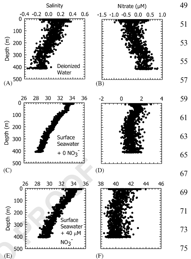
Fig. 4. Vertical profiles to 400 m with calibration solutions on retroreflection probe tip. Only the down casts are shown. (A) Salinity calculated with deionized water solution, (B) nitrate calculated with deionized water solution, (C) salinity calculated from bromide concentration in a surface seawater sample, (D) nitrate calculated in surface seawater sample, (E) salinity calculated in surface seawater sample with 40 \mu\text{M} nitrate added, and (F) nitrate calculated in surface seawater with 40 \mu\text{M} nitrate added.
